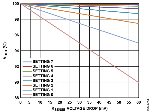
Figure 43. Load Line Settings with 60 mV CS2 Range
