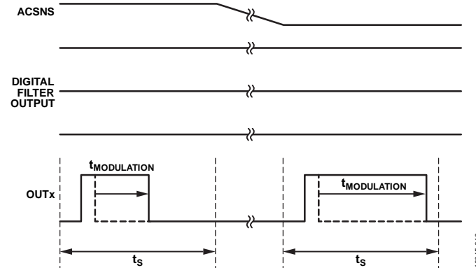
Figure 19. Feedforward Control on Modulation
