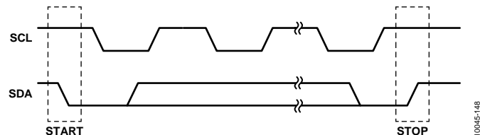
Figure 53. Start and Stop Transitions
